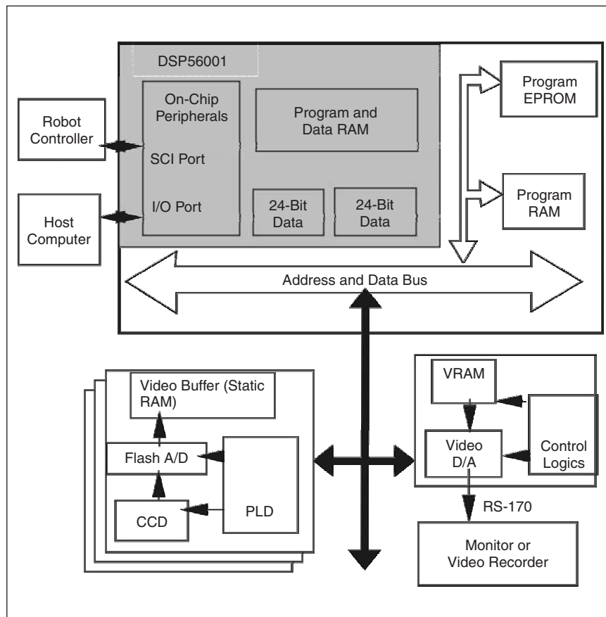
Figure 6. Schematic of a flexible integrated vision system.
