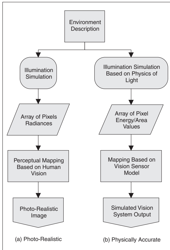
Figure 9. Model of the synthetic-imaging process.
